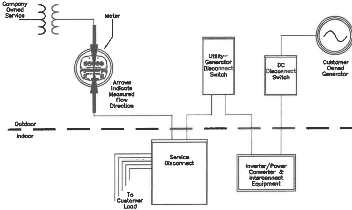
Figure 1 - Typical Residential Solar Installation
