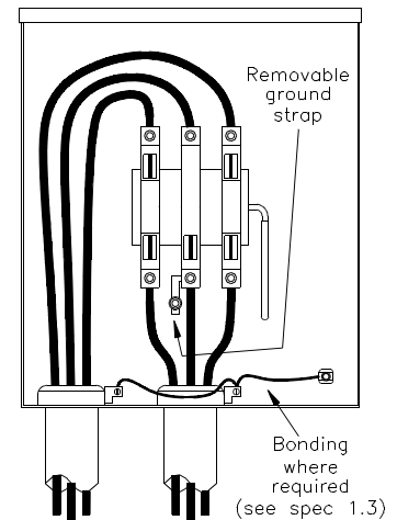
200a, 240v, 3ph, 3w
