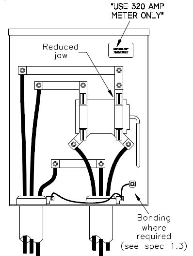
320/400a, 120/240v, 1ph, 3w
